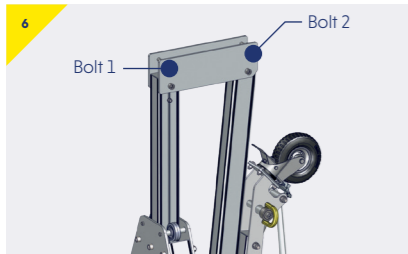
This illustration demonstrates the bolt positions (1 & 2) for the cheek plates.
